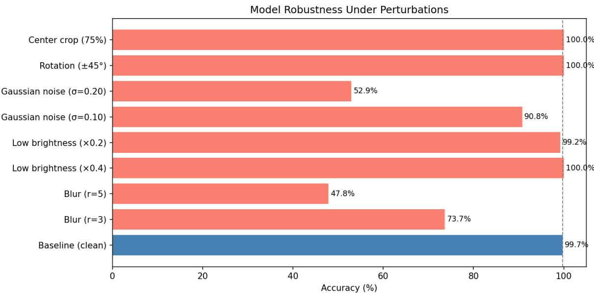
Figure 8: Model robustness under perturbations bar chart
