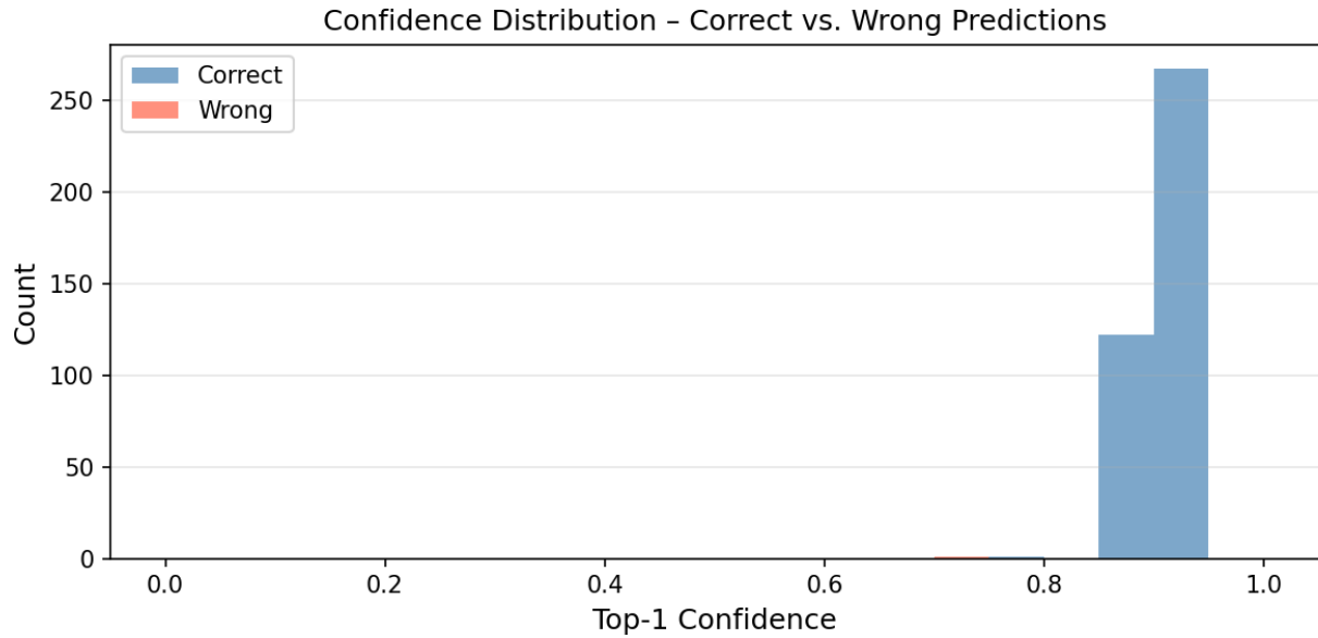
Figure 7: Confidence distribution histogram: correct vs. incorrect predictions
