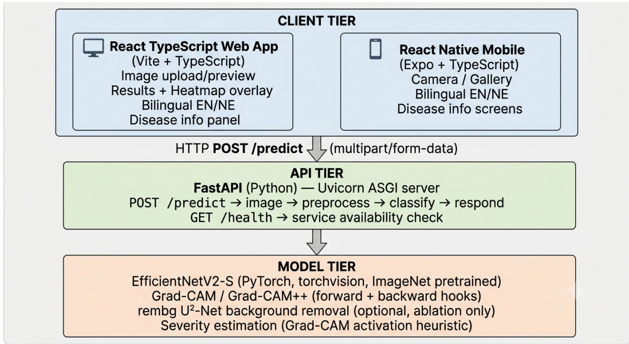
Figure 1: System architecture: three-tier client–server design.
