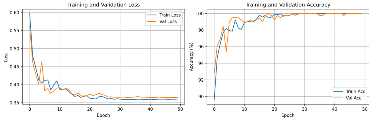
Figure 3: Training and validation loss curves over 50 epochs
